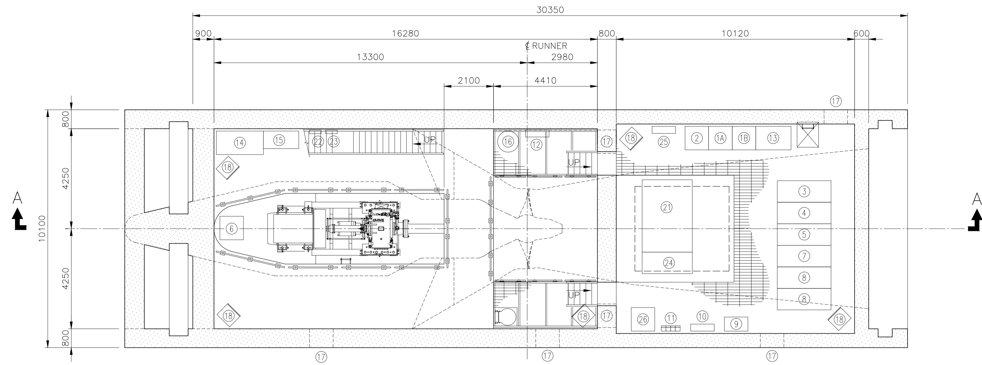
PLAN SCALE 1:100
